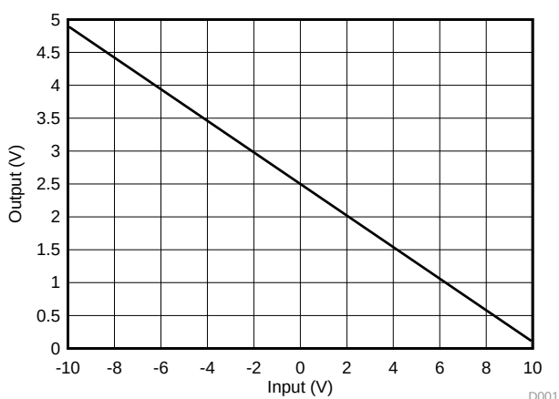
Figure 56. Plot of PLC Input Transfer Function
