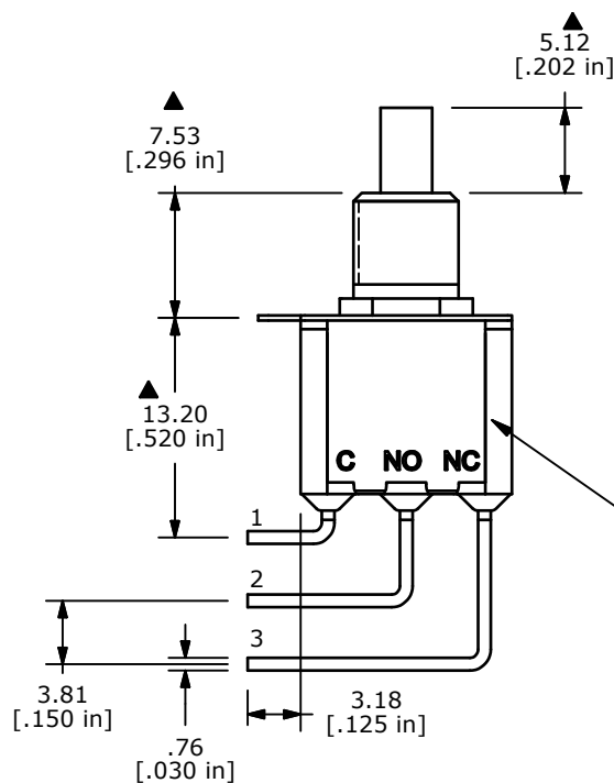
PCB MOUNTING LAYOUT
