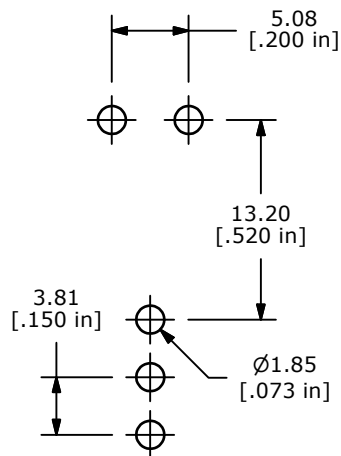
PCB MOUNTING LAYOUT
