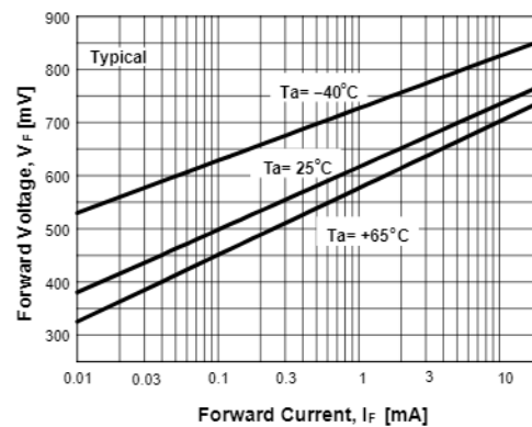
Figure 6. Forward Voltage vs. Ambient Temperature V_F - 0.01 - 20 mA (-40 \text{ to } +65^\circ C)
