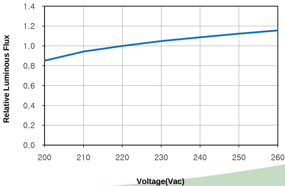
Relative Luminous Flux vs. Voltage at Ta=25℃
