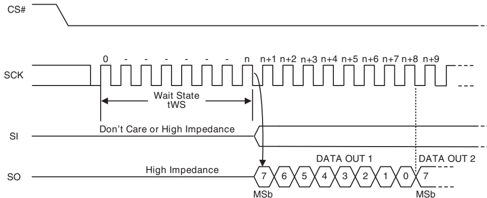
Figure 64. AutoBoot Sequence (CR1[1]=0)
