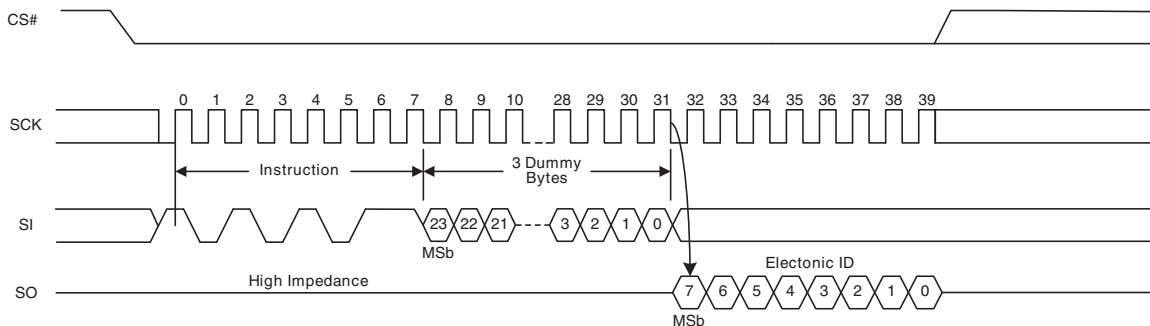
Figure 51. Read Electronic Signature (RES) Command Sequence
