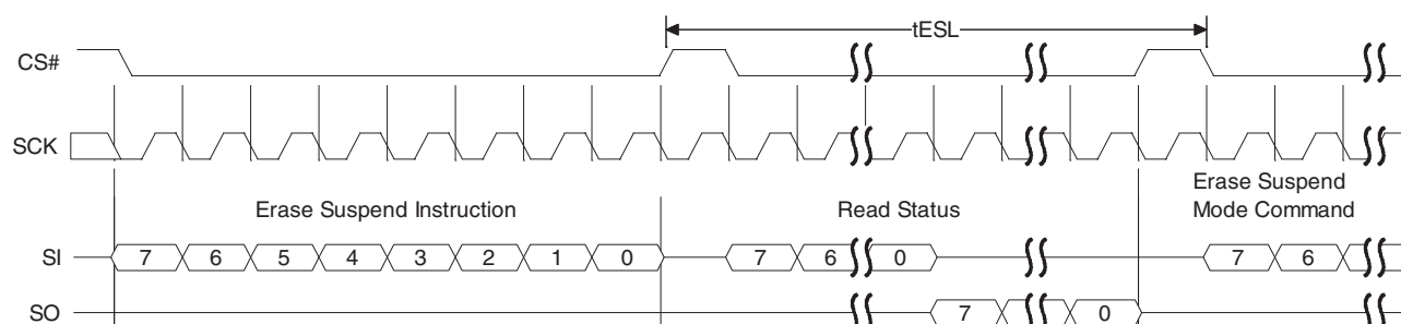
Figure 115. Erase Suspend Command Sequence
