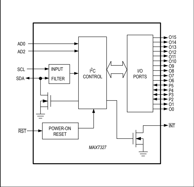
Functional Diagram
