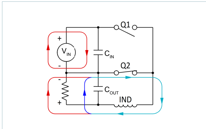
Figure 65 — Current flow: Q2 closed
