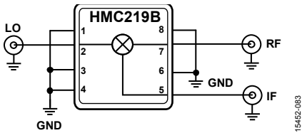
Figure 83. Typical Application Circuit
