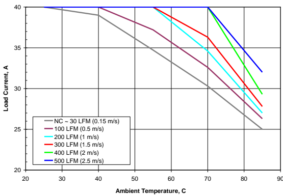
Figure 1. Available load current vs. ambient air temperature and airflow rates for SQE48T40015 converter mounted vertically with air flowing from pin 3 to pin 1, MOSFET temperature \leq 120\text{ }^\circ\text{C} , V_{in} = 48\text{ V} . Note: NC – Natural convection
