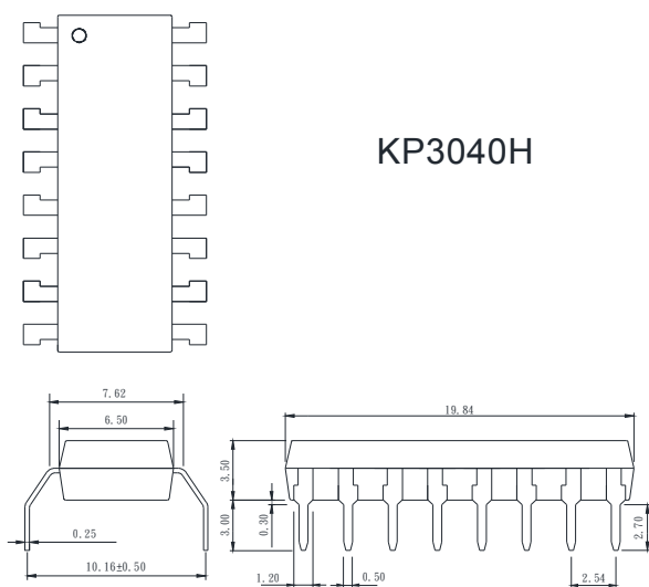
3. Long creepage distance type
