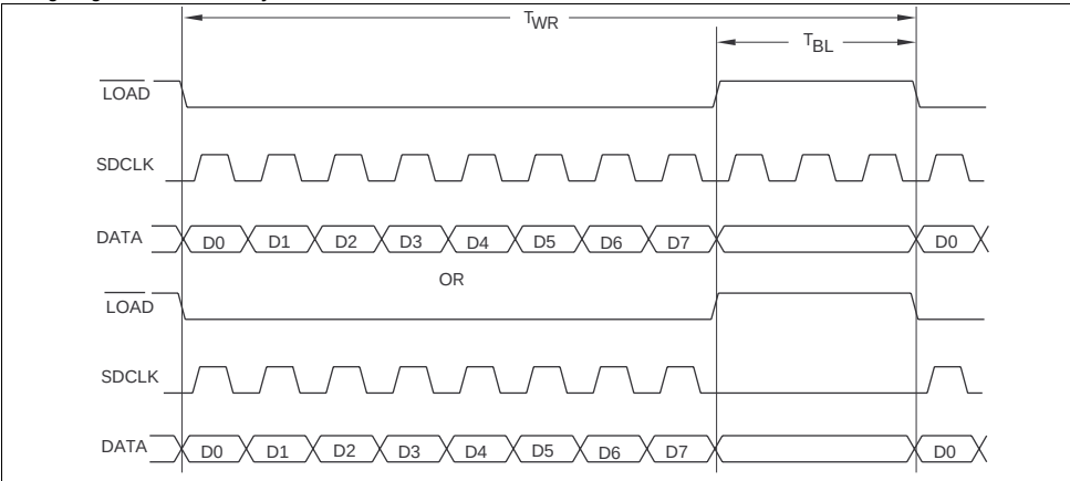
Timing Diagram—Instruction Cycle
