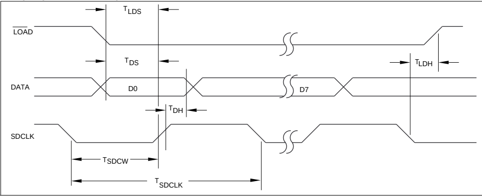
Timing Diagram—Data Write Cycle
