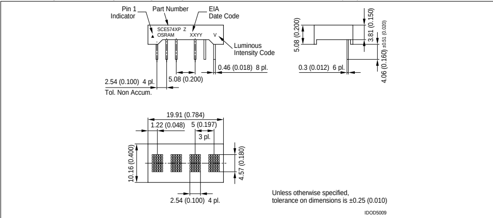
Detail Drawing of SCE574xQ (SIP configuration with right angle bend)
