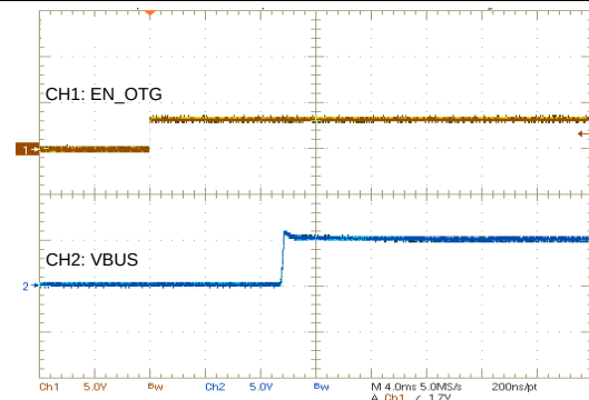
图 61. OTG Power Up from 8 V Battery
