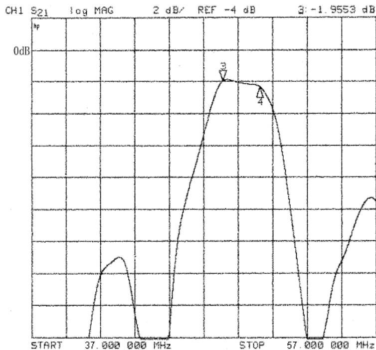
Transfer function channel 48 (pass band):
