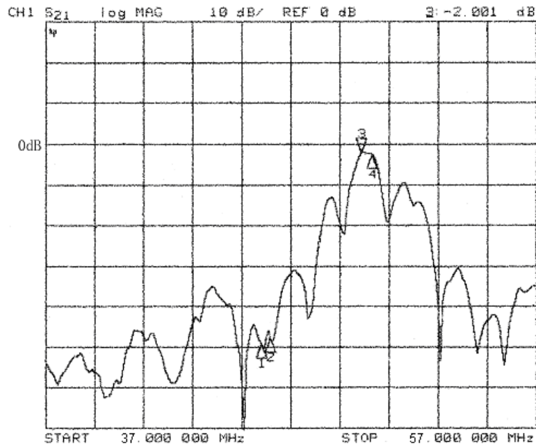
Transfer function channel 48:
