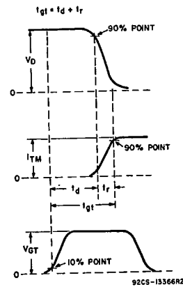
Fig. 11 — Relationship between off-state voltage, on-state current, and gate-trigger voltage showing reference points for definition of turn-on time ( t_{gu} ).
