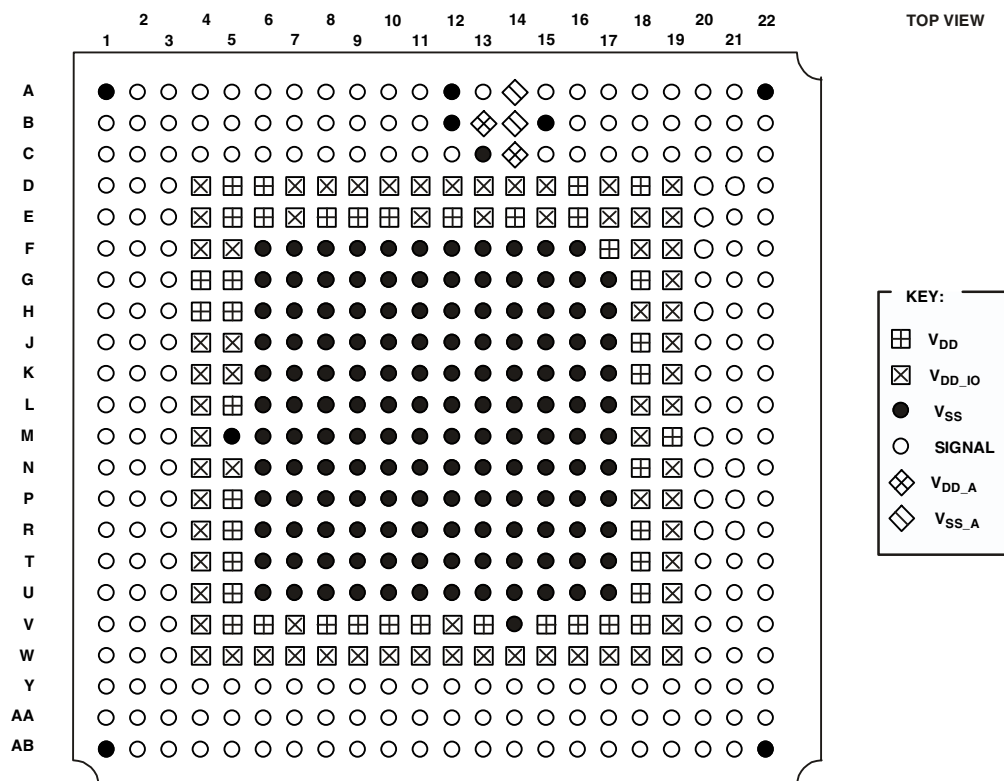
Figure 40. 484-Ball PBGA Pin Configurations (Top View, Summary)
