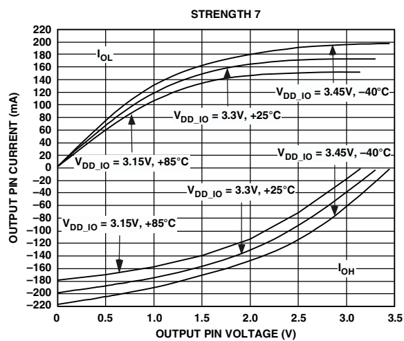
Figure 27. Typical Drive Currents at Strength 7
