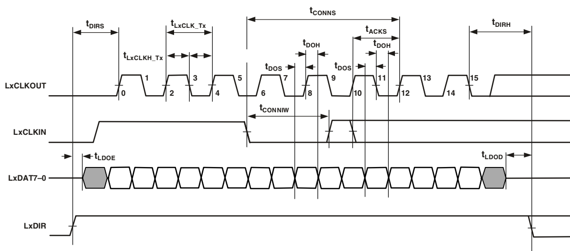
Figure 16. Link Ports—Transmit
