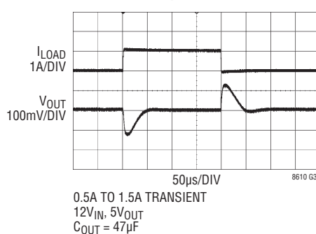
Transient Response
