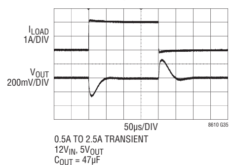
Transient Response
