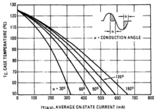
FIGURE 3 – AVERAGE CURRENT DERATING (REFERENCE: CASE TEMPERATURE)
