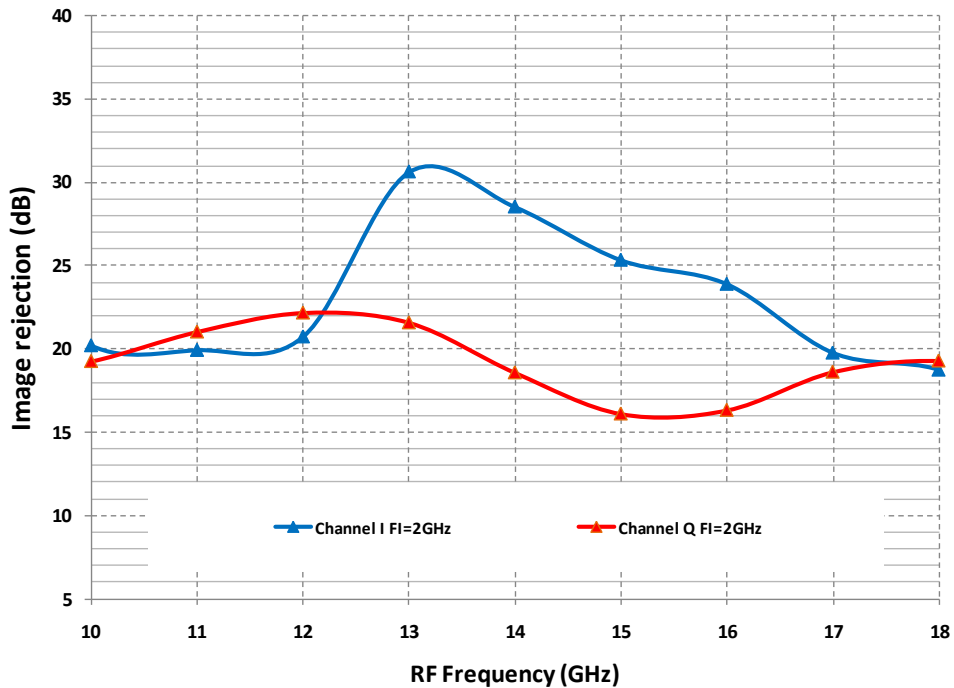
Image Rejection versus frequency RF = LO+/- IF, IF = 2GHz, GC = -1.5V
