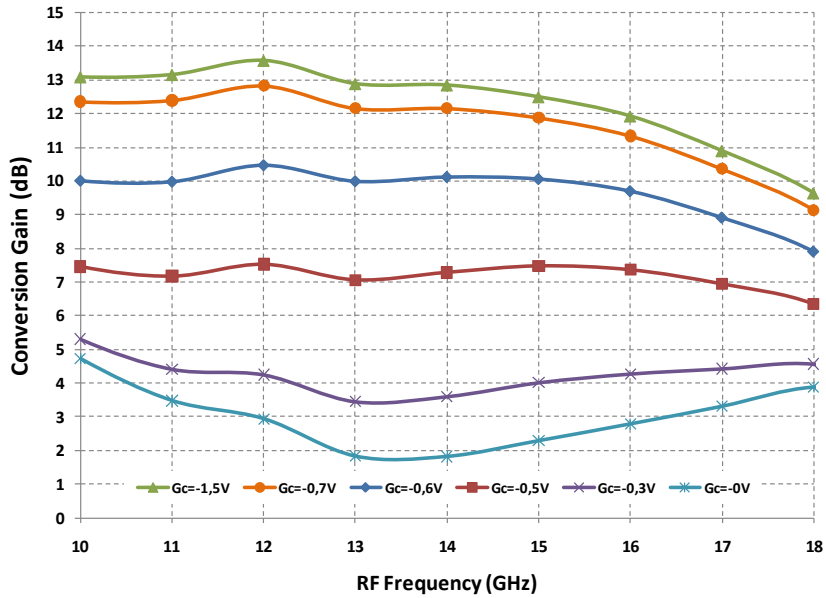
Conversion Gain in Supradynne Mode versus RF Frequency & GC RF = LO+ IF, IF = 2GHz
