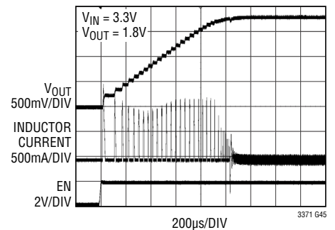
4A Buck Regulator No-Load Startup Transient (Forced Continuous Mode)
