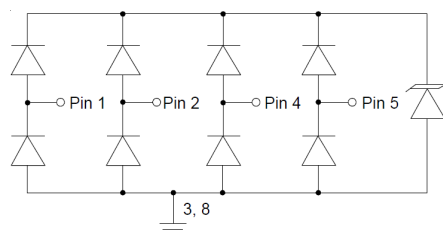
DFN2510-10L
