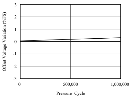
Offset Voltage Variation
