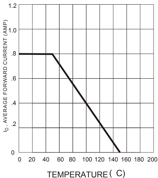
FIG.1 CURRENT DERATING
