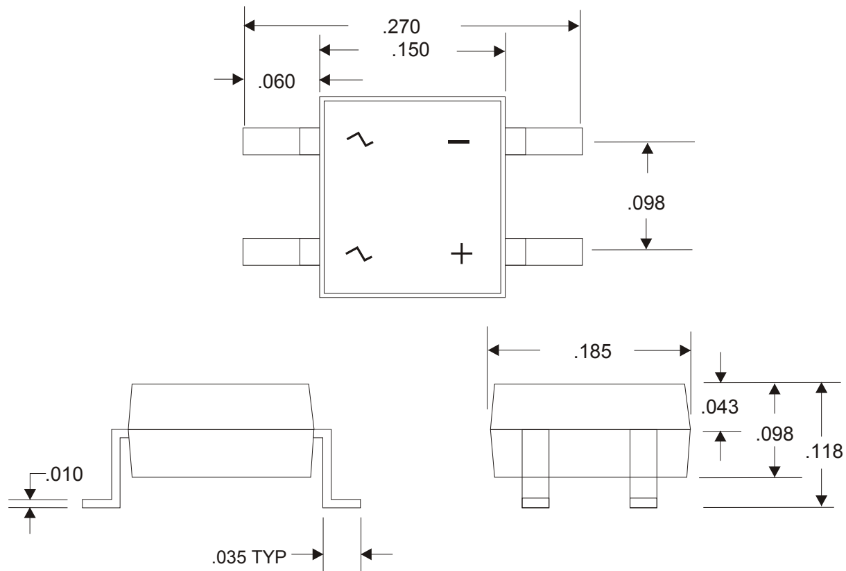
FIG.3 MECHANICAL DIMENSIONS
