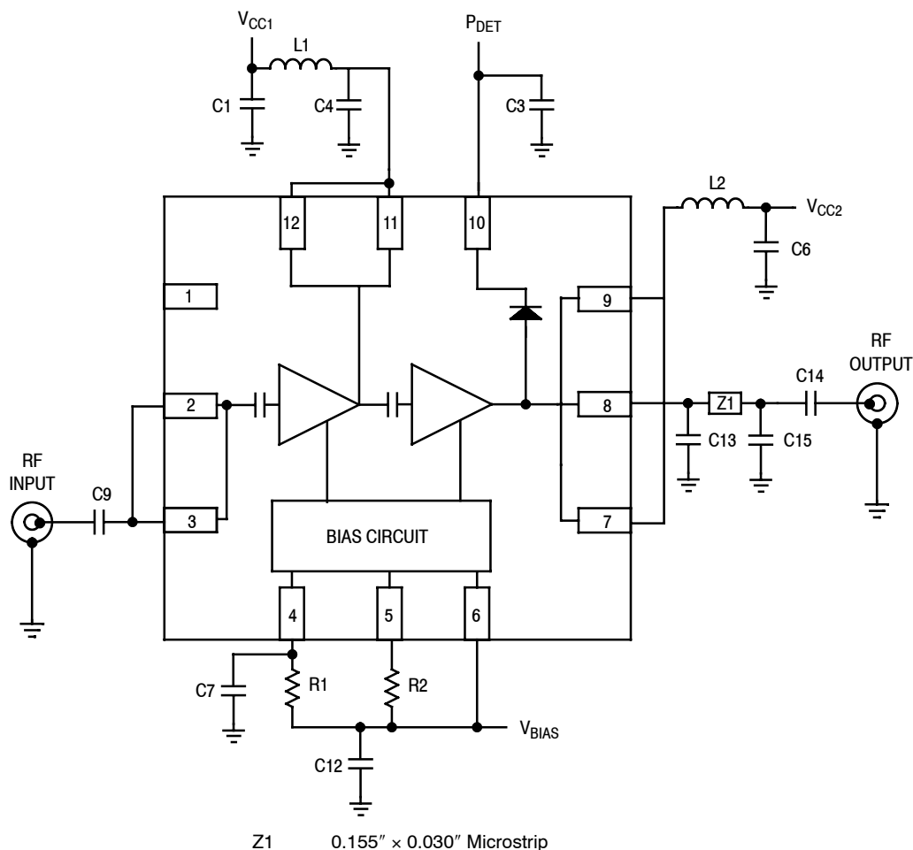
Figure 3. MMZ25332BT1 Test Circuit Schematic — 2500 MHz, 5 Volt Operation
