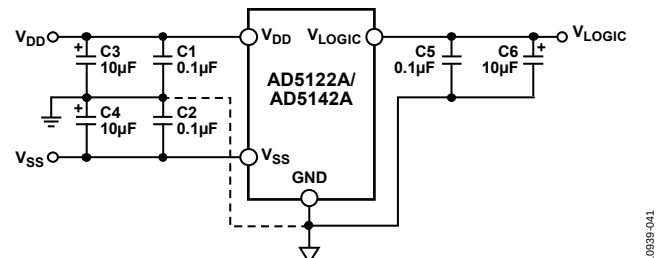
Figure 42. Power Supply Bypassing
