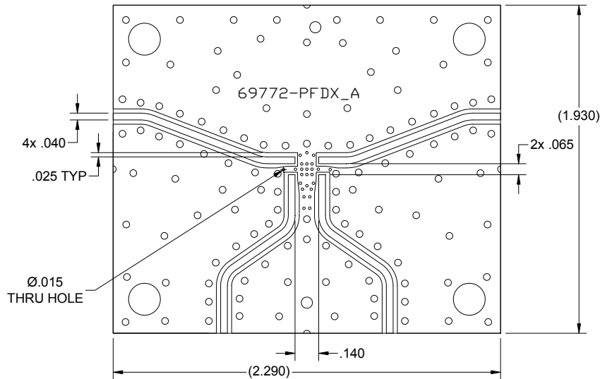
10dB, 20dB and 30dB Test Board
