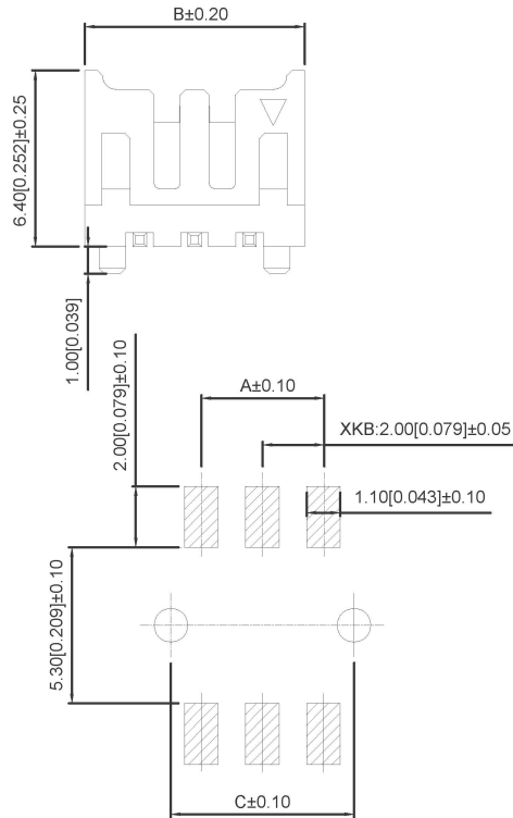
PCB LAYOUT
