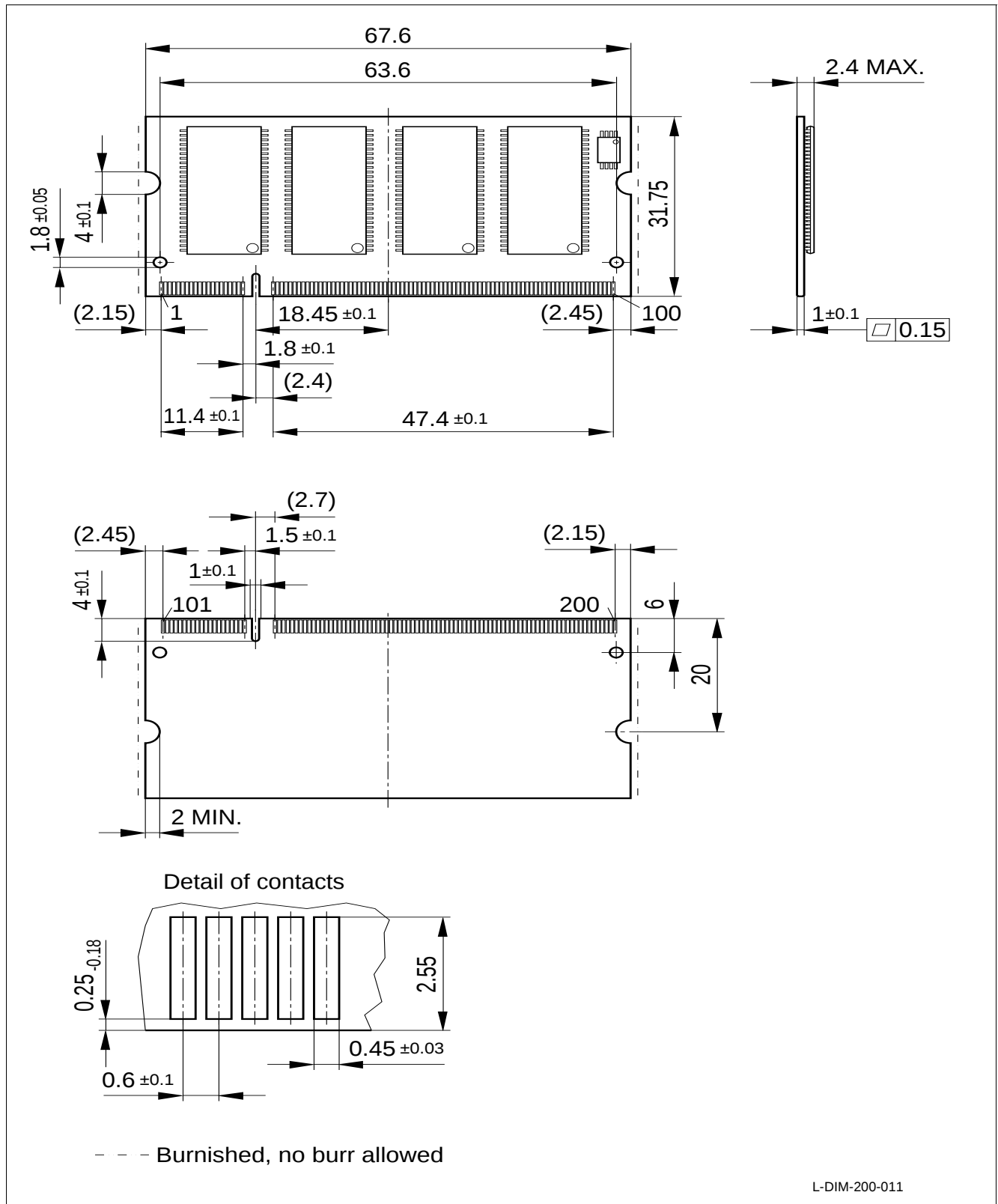
Figure 4 Package Outlines – Raw Card C DDR-SDRAM SO-DIMM HYS64D16000HDL-6-C
