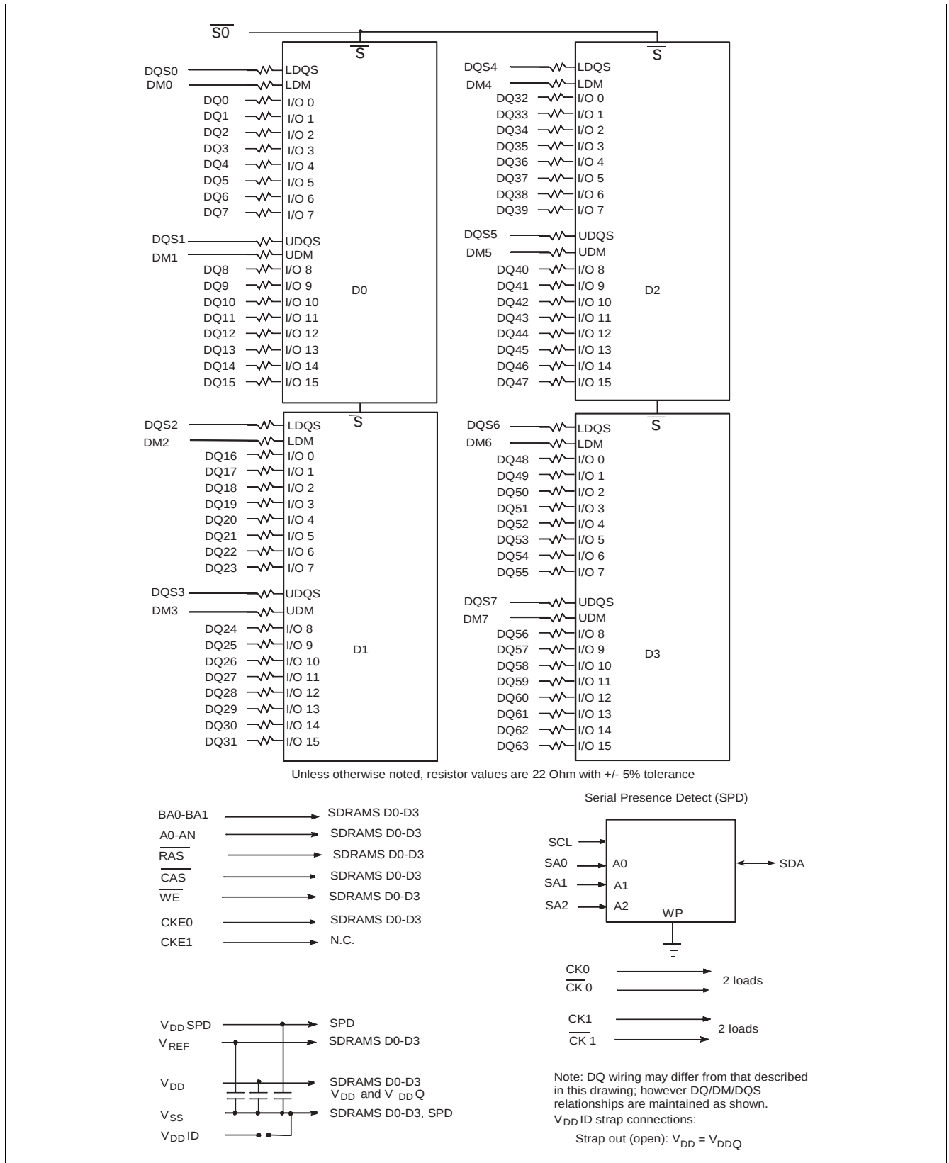
Figure 2 Block Diagram - One Rank 16M x 64 DDR SDRAM SO-DIMM HYS64D16000HDL-6-C
