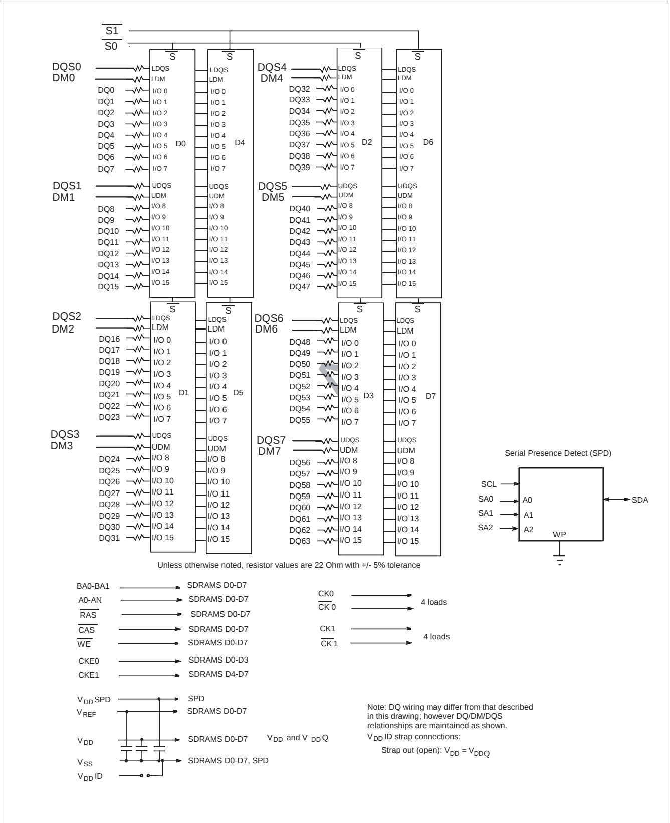
Figure 3 Block Diagram - Two Ranks 32M × 64 DDR SDRAM SO-DIMM HYS64D32020HDL-6-C
