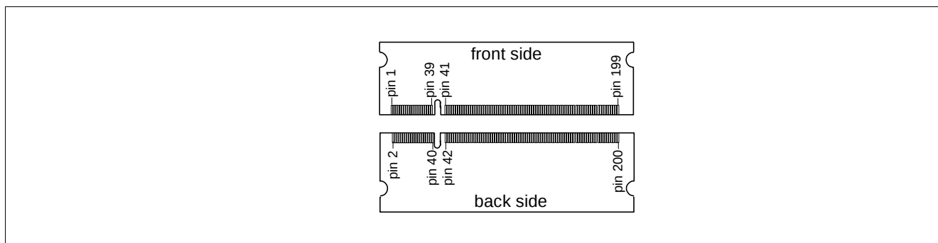
Figure 1 Pin Configuration
