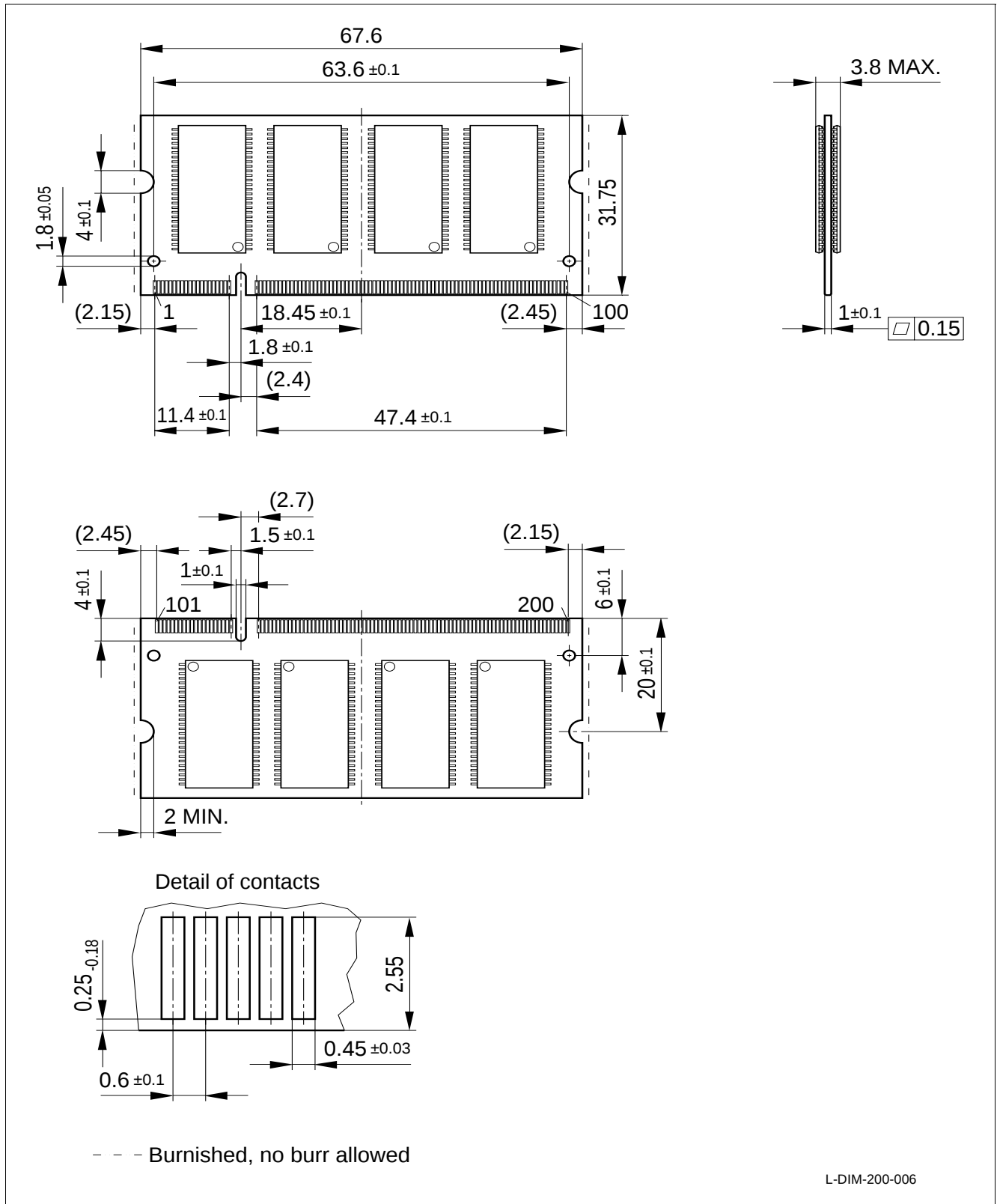
Figure 5 Package Outlines – Raw Card A DDR SDRAM SO-DIMM HYS64D32020HDL-6-C
