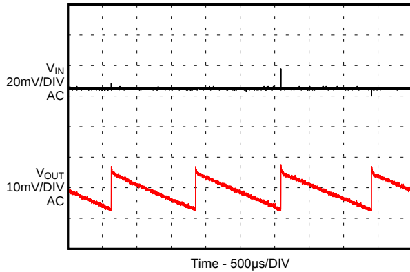
图 24. Input and Output Ripple in PSM Mode
