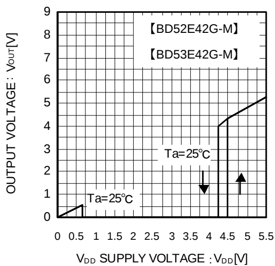
Figure.6 I/O Characteristics
