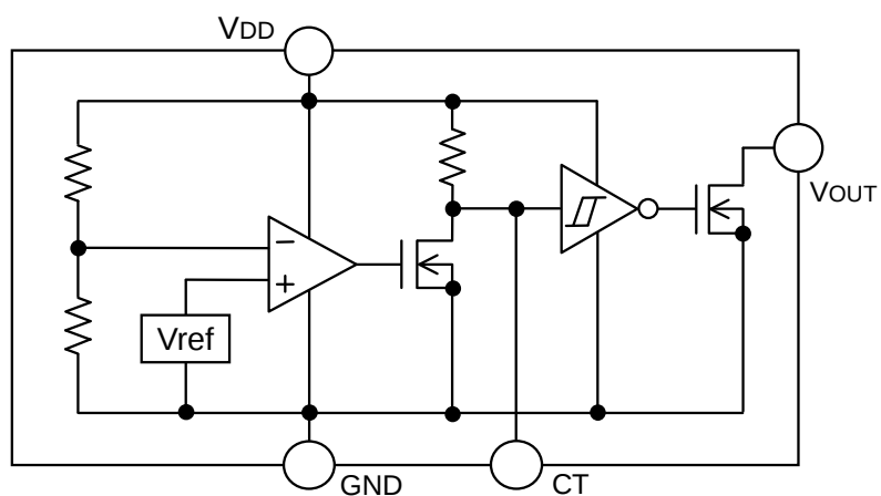
Figure.1 BD52Exxx-M Series
