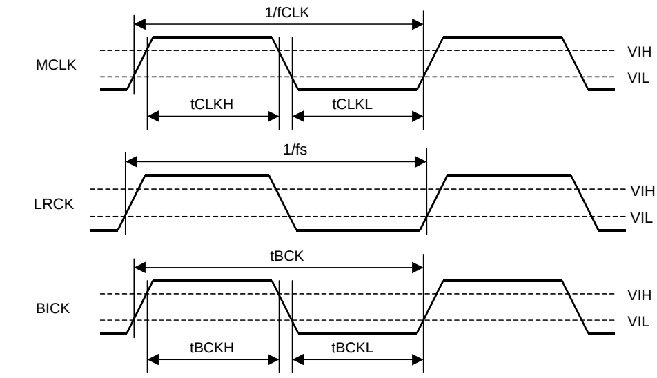
Clock Timing
