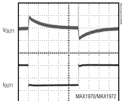
LOAD-TRANSIENT RESPONSE
