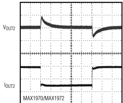
LOAD-TRANSIENT RESPONSE
