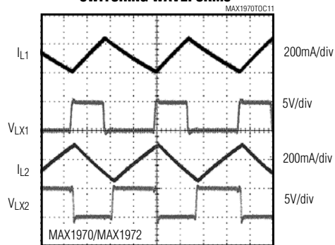
SWITCHING WAVEFORMS
