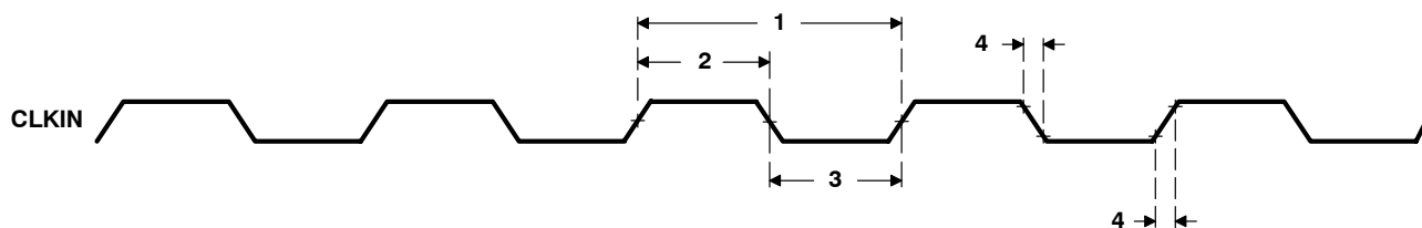
Figure 15. CLKIN Timings
