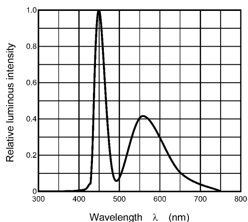
Fig. 8.6 Wavelength Characteristic
