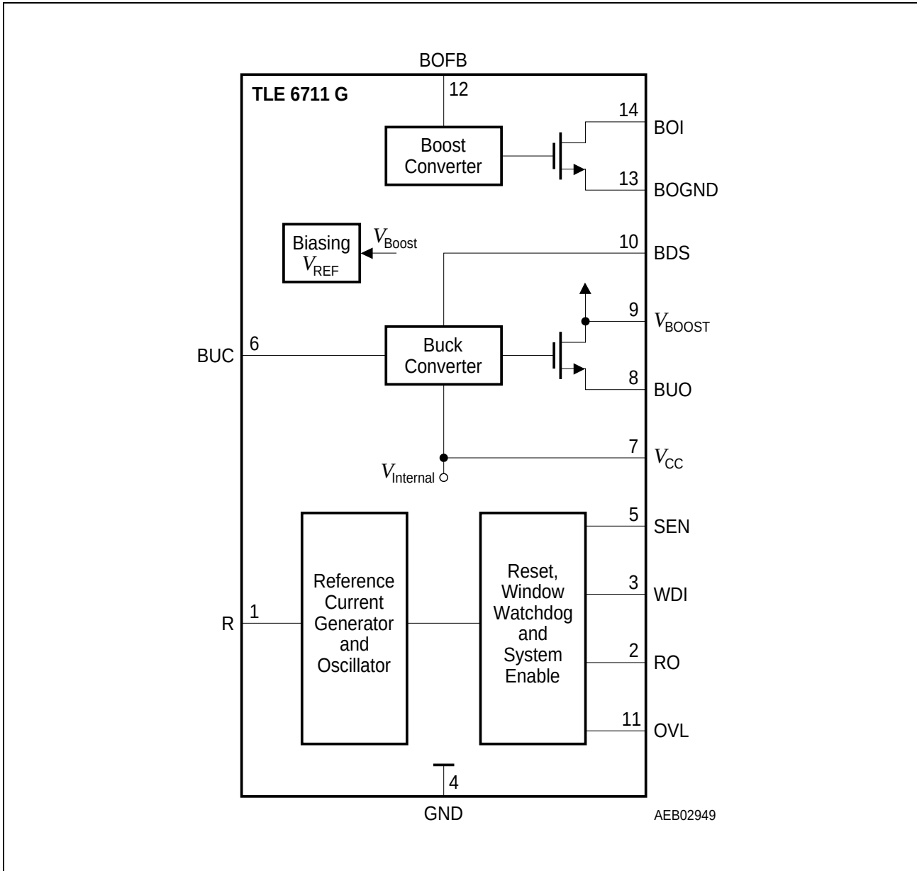
Figure 2 Block Diagram
