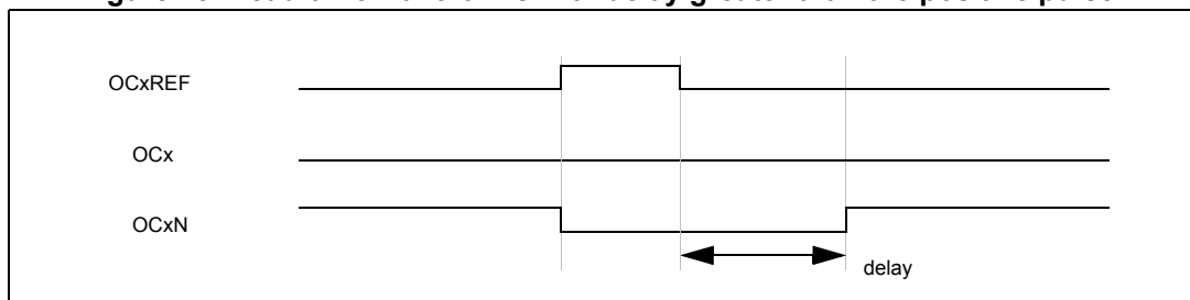
Figure 75. Dead-time waveforms with delay greater than the positive pulse.
