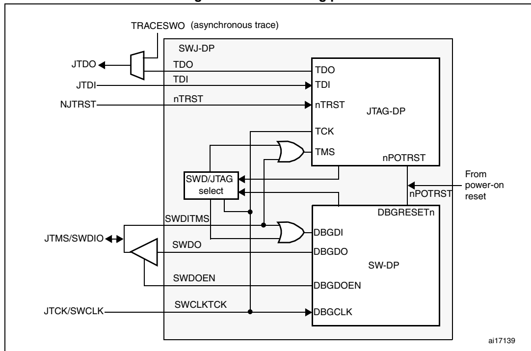
Figure 267. SWJ debug port
