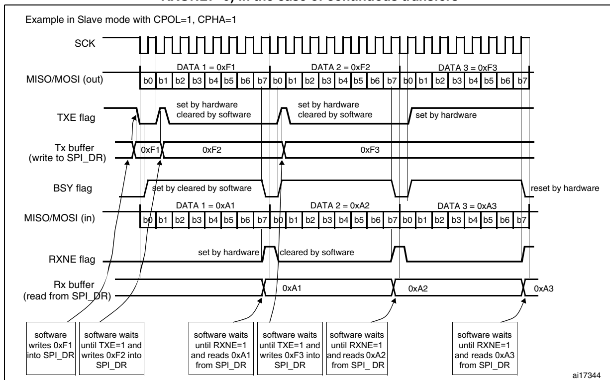
Figure 200. TXE/RXNE/BSY behavior in Slave / full-duplex mode (BIDIMODE=0, RXONLY=0) in the case of continuous transfers
