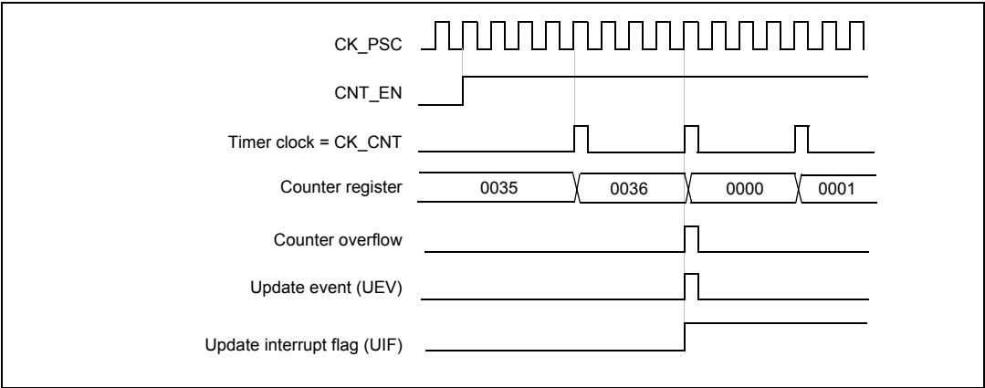
Figure 44. Counter timing diagram, internal clock divided by 4
