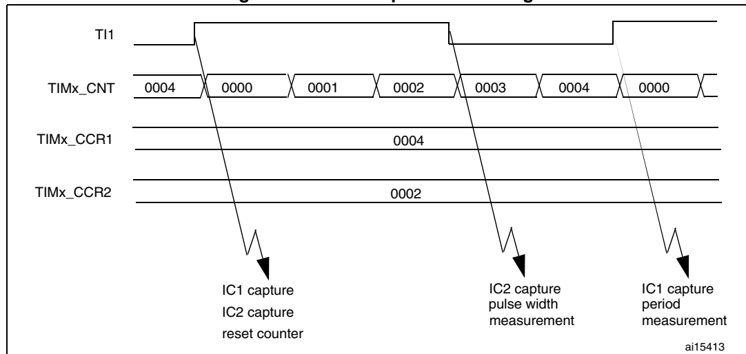
Figure 149. PWM input mode timing
