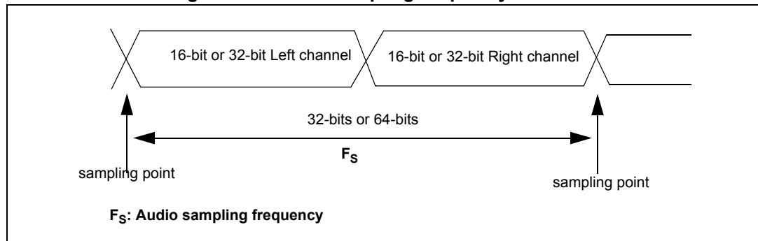
Figure 227. Audio sampling frequency definition
