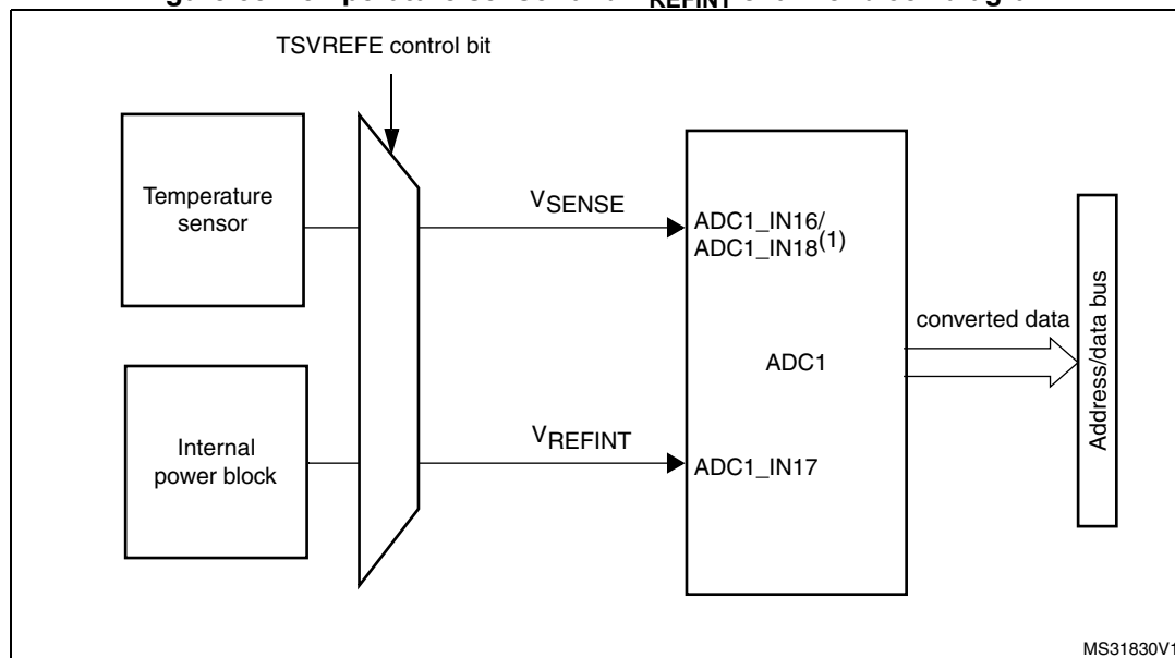
Figure 38. Temperature sensor and V_{REFINT} channel block diagram
