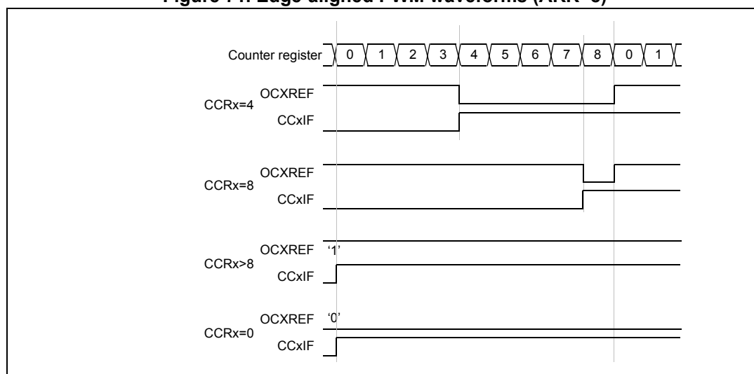
Figure 71. Edge-aligned PWM waveforms (ARR=8)
