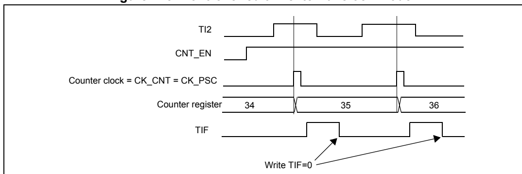
Figure 145. Control circuit in external clock mode 1
