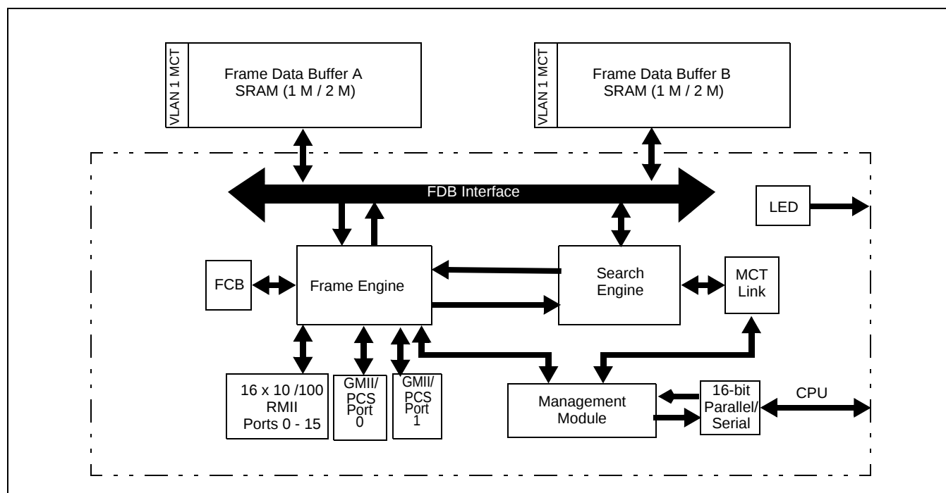
Figure 1 - ZL50418 System Block Diagram
