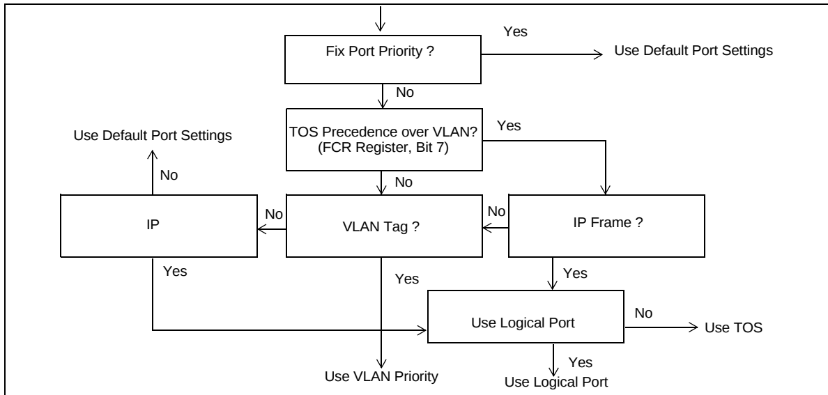
Figure 8 - Priority Classification Rule
