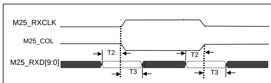
Figure 30 - Gigabit TBI Interface Receive Timing
