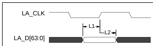
Figure 21 - Local Memory Interface – Input Setup and Hold Timing
