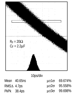
RECOVERED CLOCK JITTER (155Mbps, 1-0 PATTERN, 4.7ps RMS)
