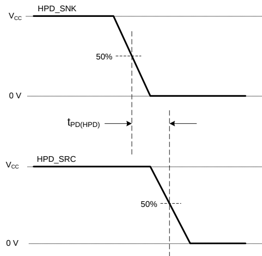
Figure 10. HPD Timing Diagram Number 1
