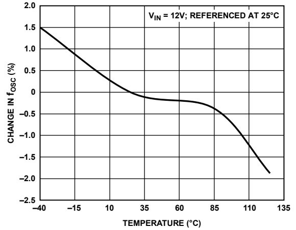
Figure 20. f_{osc} vs. Temperature
