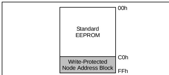
FIGURE 3-1: MEMORY ORGANIZATION
