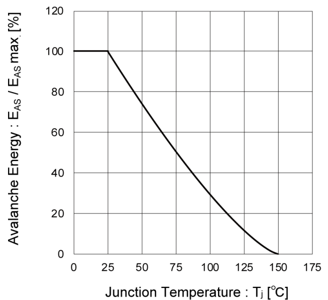
Fig.3 Avalanche Energy Drating Curve vs. Junction Temperature
