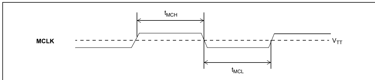
Figure 17 - Master Clock
