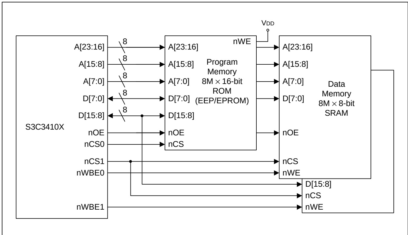
Figure 4-17. 8MB × 16 Program Memory &amp; two 8MB × 8 Data Memory
