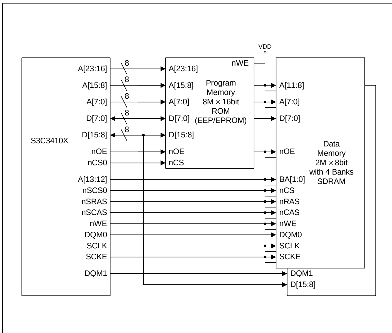
Figure 4-22. 8MB × 16 Program Memory &amp; two 2MB × 8 with 4 Banks SDRAM
