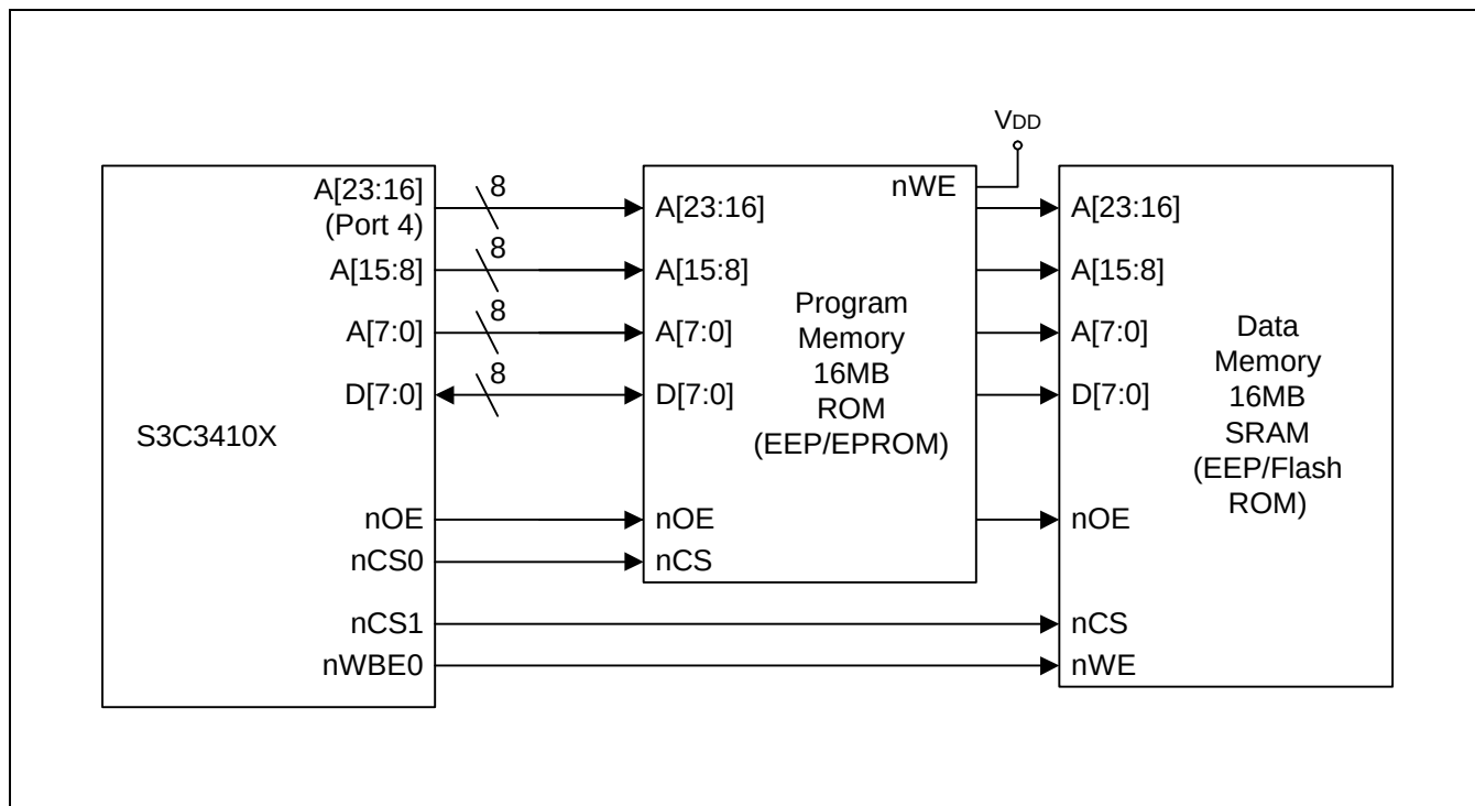
Figure 4-16. 16MB x 8 Program Memory &amp; 16MB x 8 Data Memory
