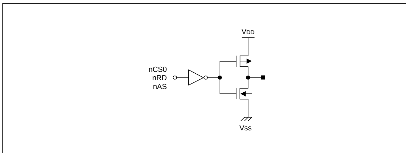
Figure 7-16. Pin Circuit Type 10 (nCS0, nRD and nAS)
