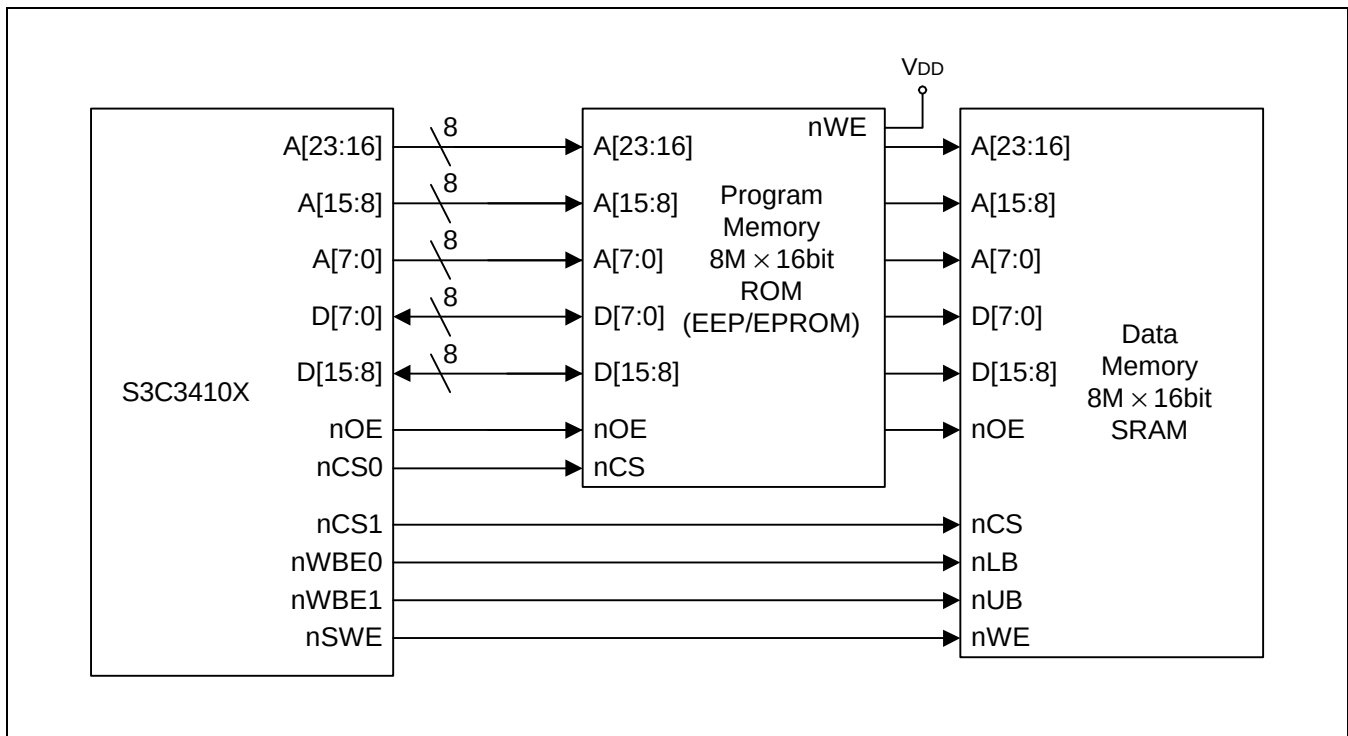
Figure 4-18. 8MB × 16 Program Memory &amp; 8MB × 16 Data Memory (SRAM)
