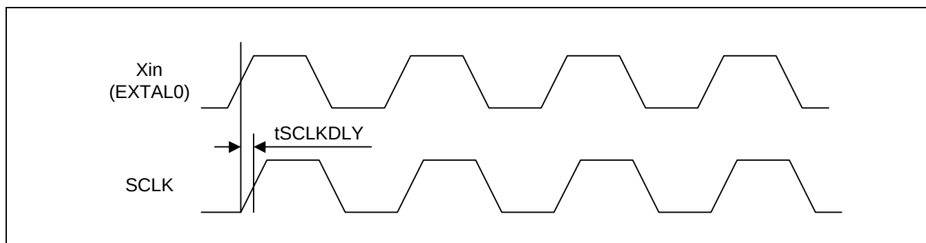
Figure 17-3. X_{in} (EXTAL0)/SCLK Timing
