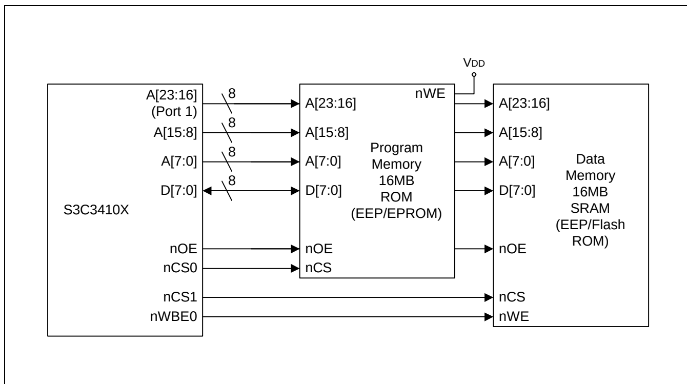
Figure 4-15. 16MB x 8 Program Memory &amp; 16MB x 8 Data Memory
