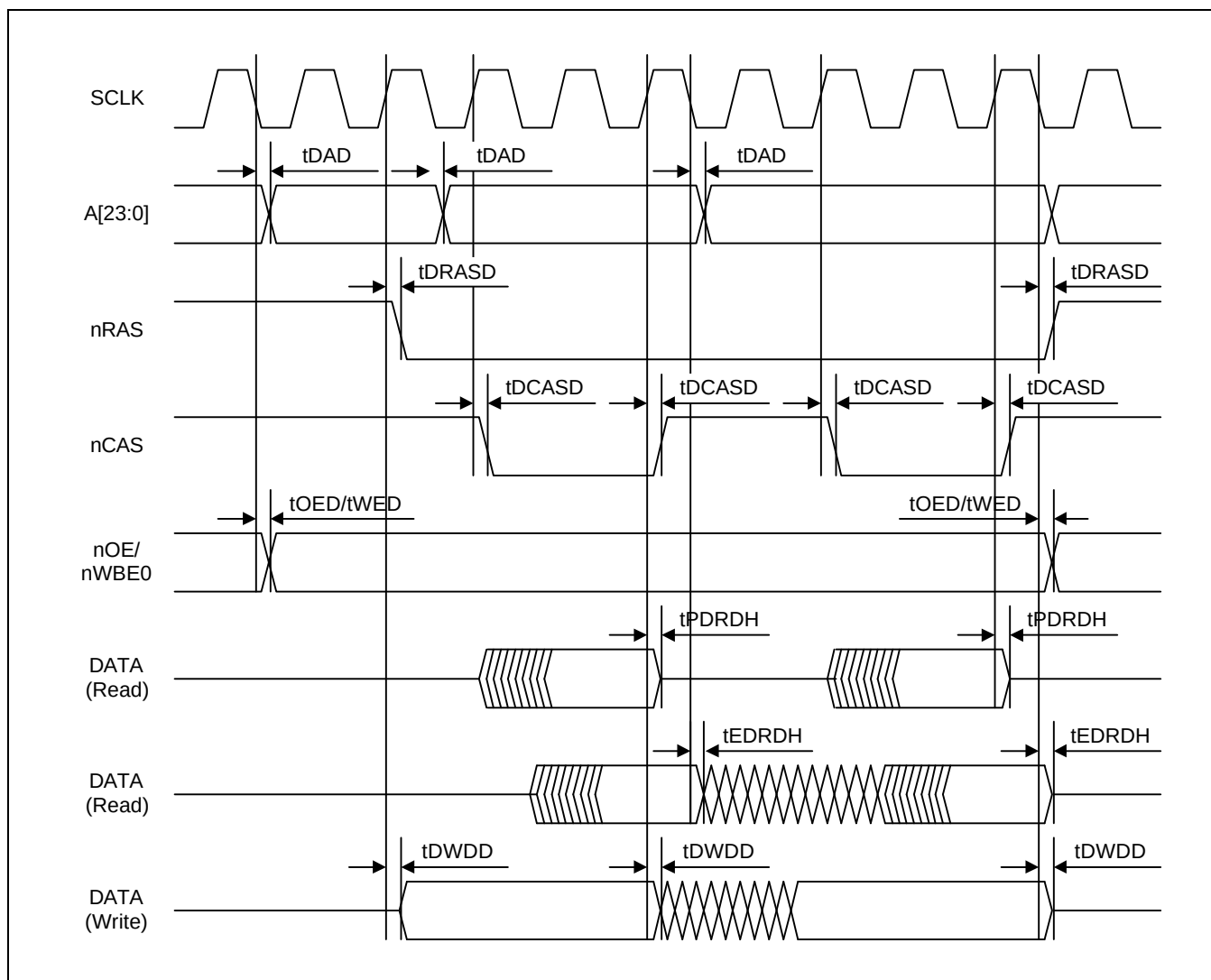
Figure 17-5. DRAM (Fast Page/EDO) Bus Timing
