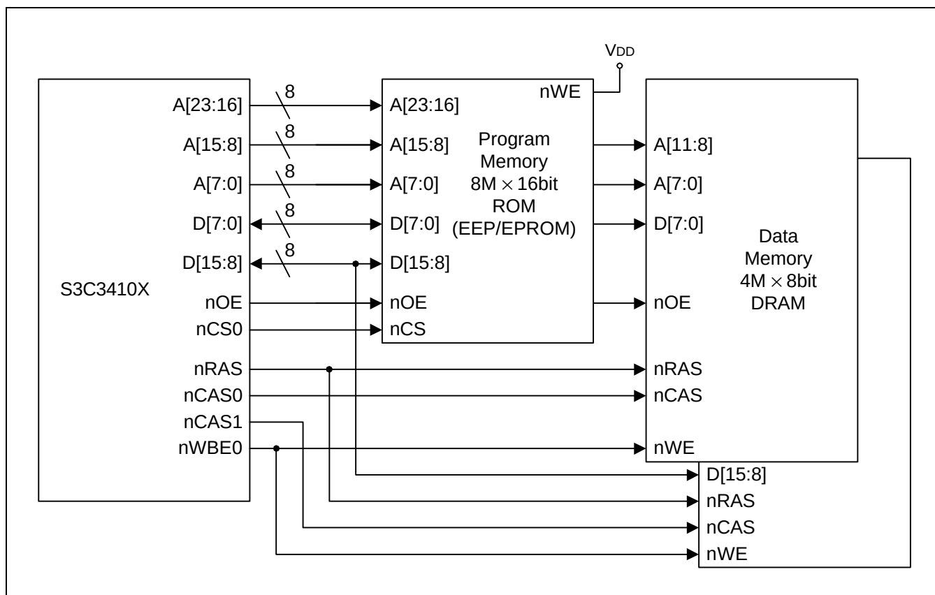
Figure 4-19. 8MB × 16 Program Memory &amp; two 4MB × 8 Data Memory (DRAM)
