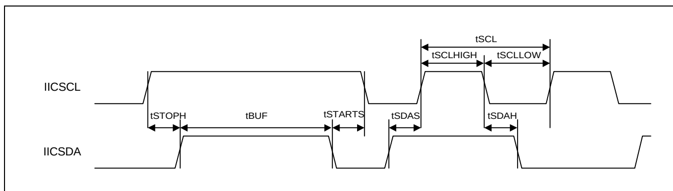
Figure 17-9. IIC Interface Timing
