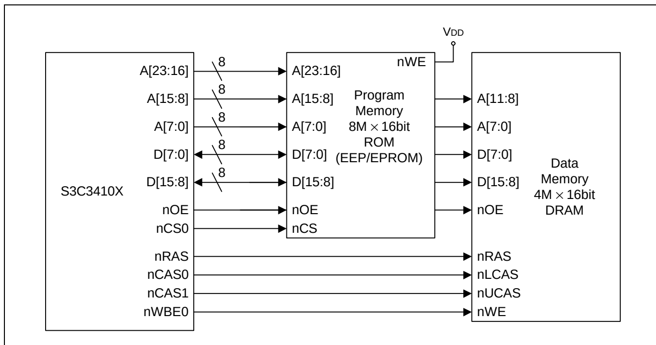
Figure 4-20. 8MB × 16 Program Memory &amp; 4MB × 16 Data Memory (DRAM)
