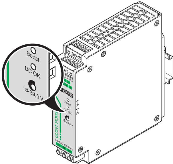
Figure 8 Signal outputs
