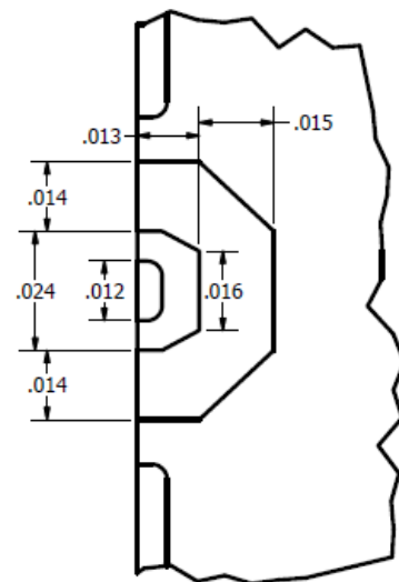
DETAIL A
