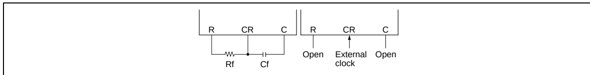
Figure 1 Oscillator Connection with HD61202U
