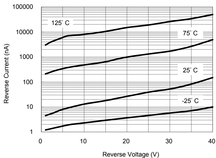
Fig. 2 Reverse Characteristics
