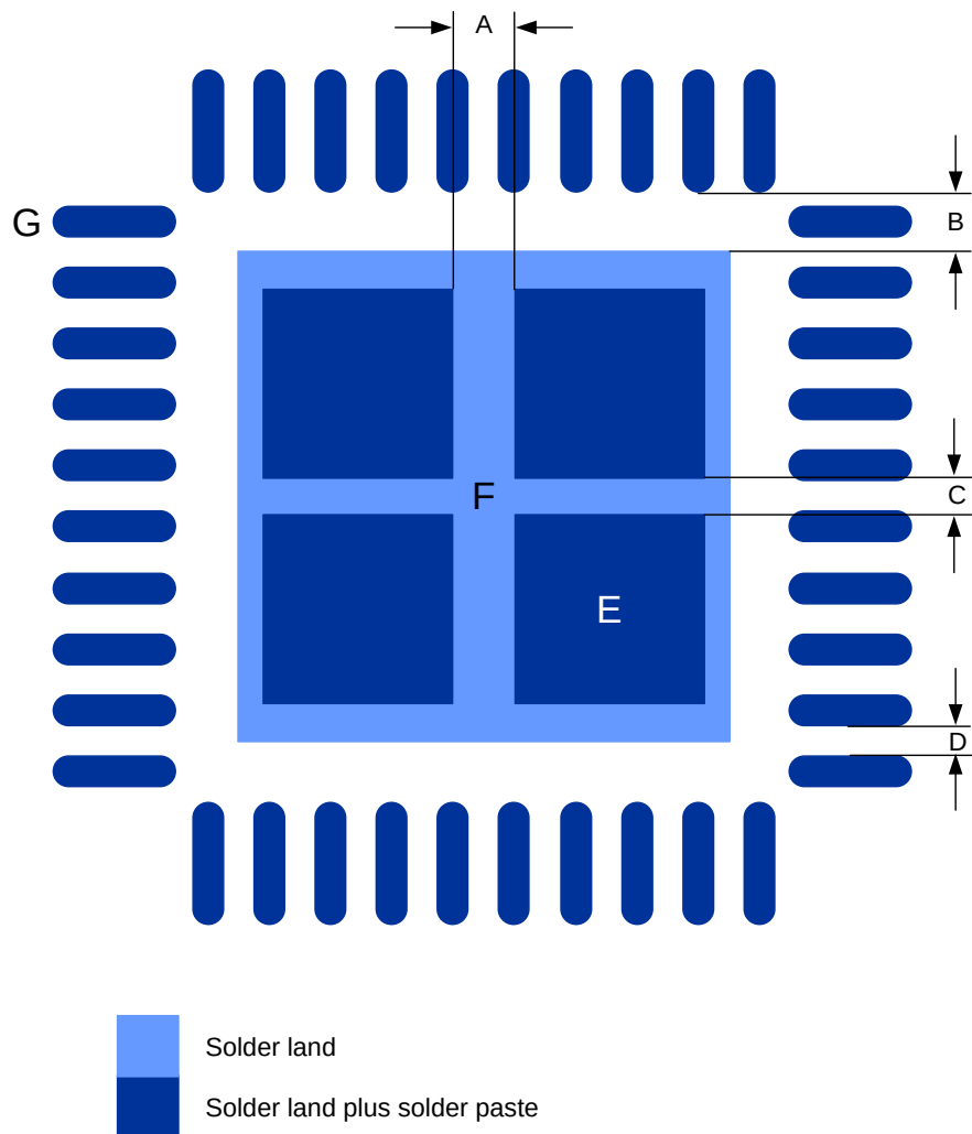
Figure 46: PCB Decal
