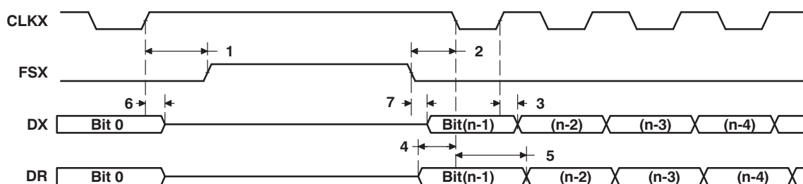
Figure 11-40. McBSP as SPI Master or Slave: CLKSTP = 11b, CLKXP = 1
