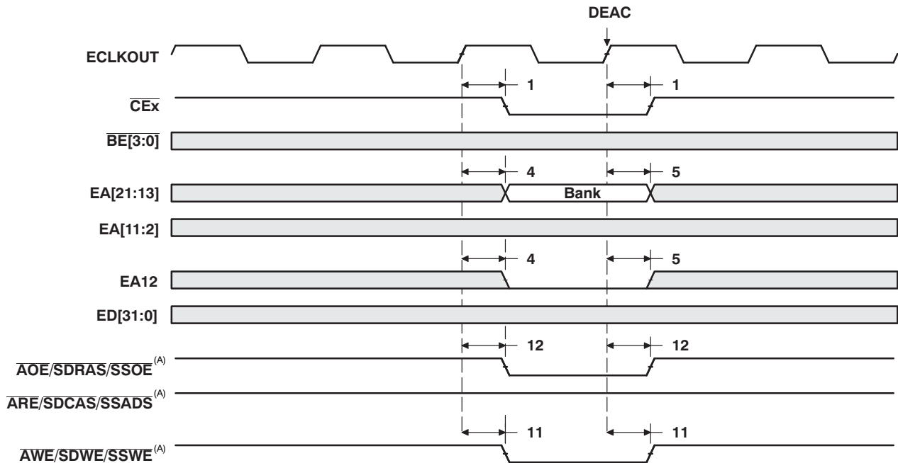
Figure 11-19. SDRAM DCAB Command
