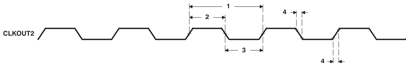
Figure 11-8. CLKOUT2
