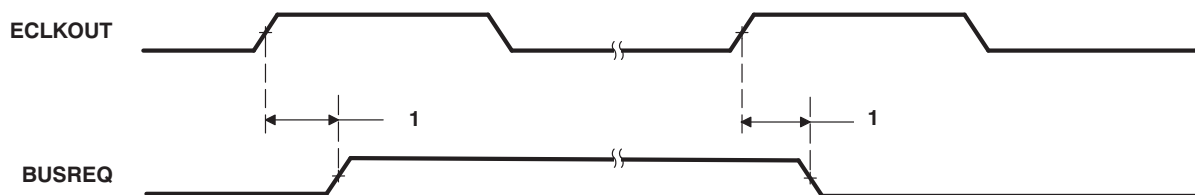
Figure 11-24. BUSREQ
