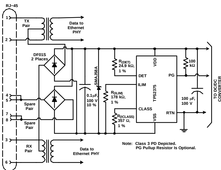
Figure 1. Typical Application Circuit and Startup Waveforms
