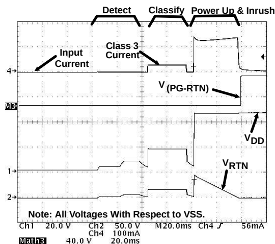
Figure 1. Typical Application Circuit and Startup Waveforms
